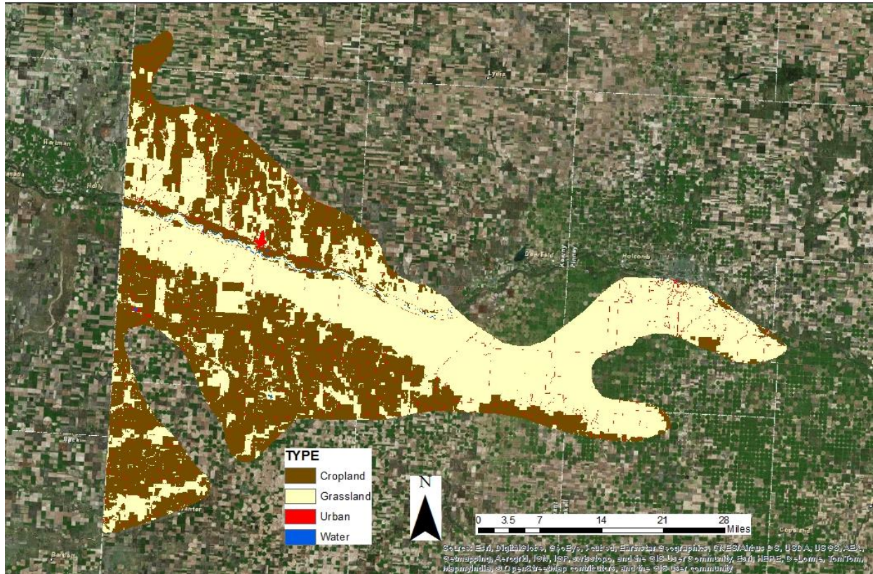
Figure 4.1 Land cover map of Range 5 in the Lesser Prairie-Chicken range during the 1960s. Much of the eastern portion of this range was continuous grassland during this time period.
